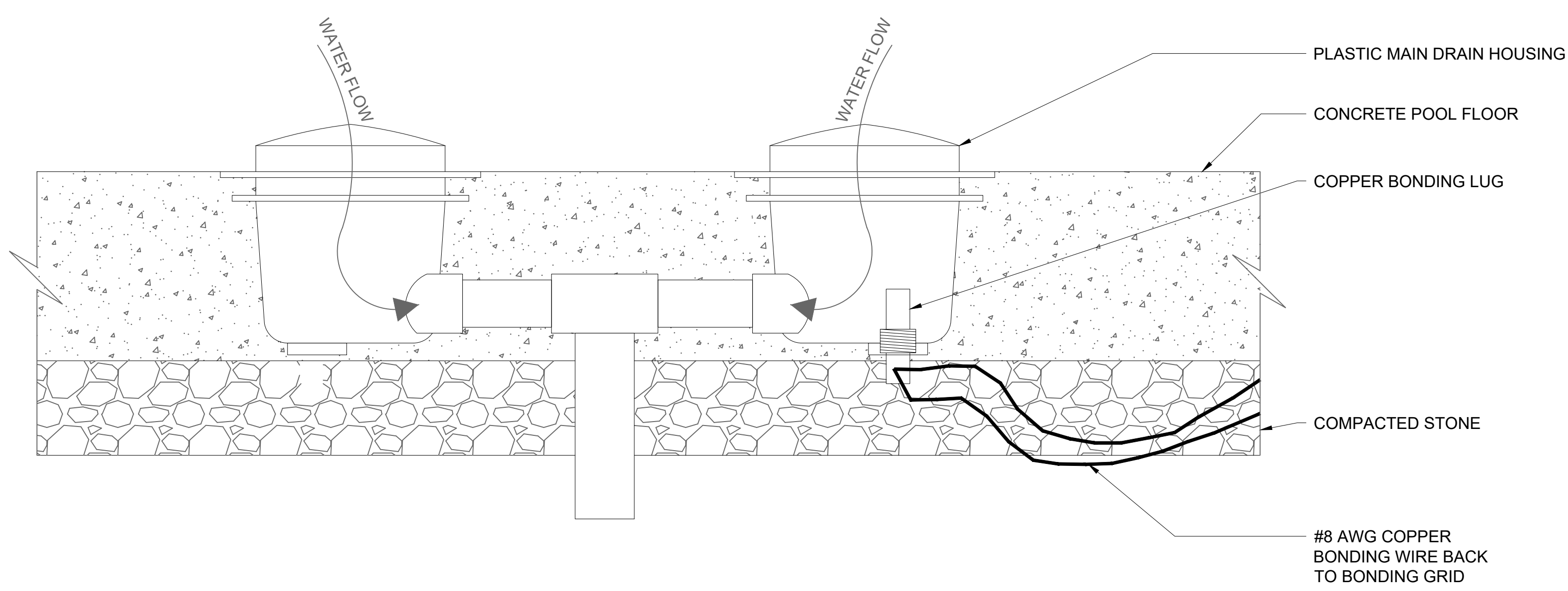
2 WATER BONDING AT MAIN DRAIN DETAIL SCALE: NOT TO SCALE
