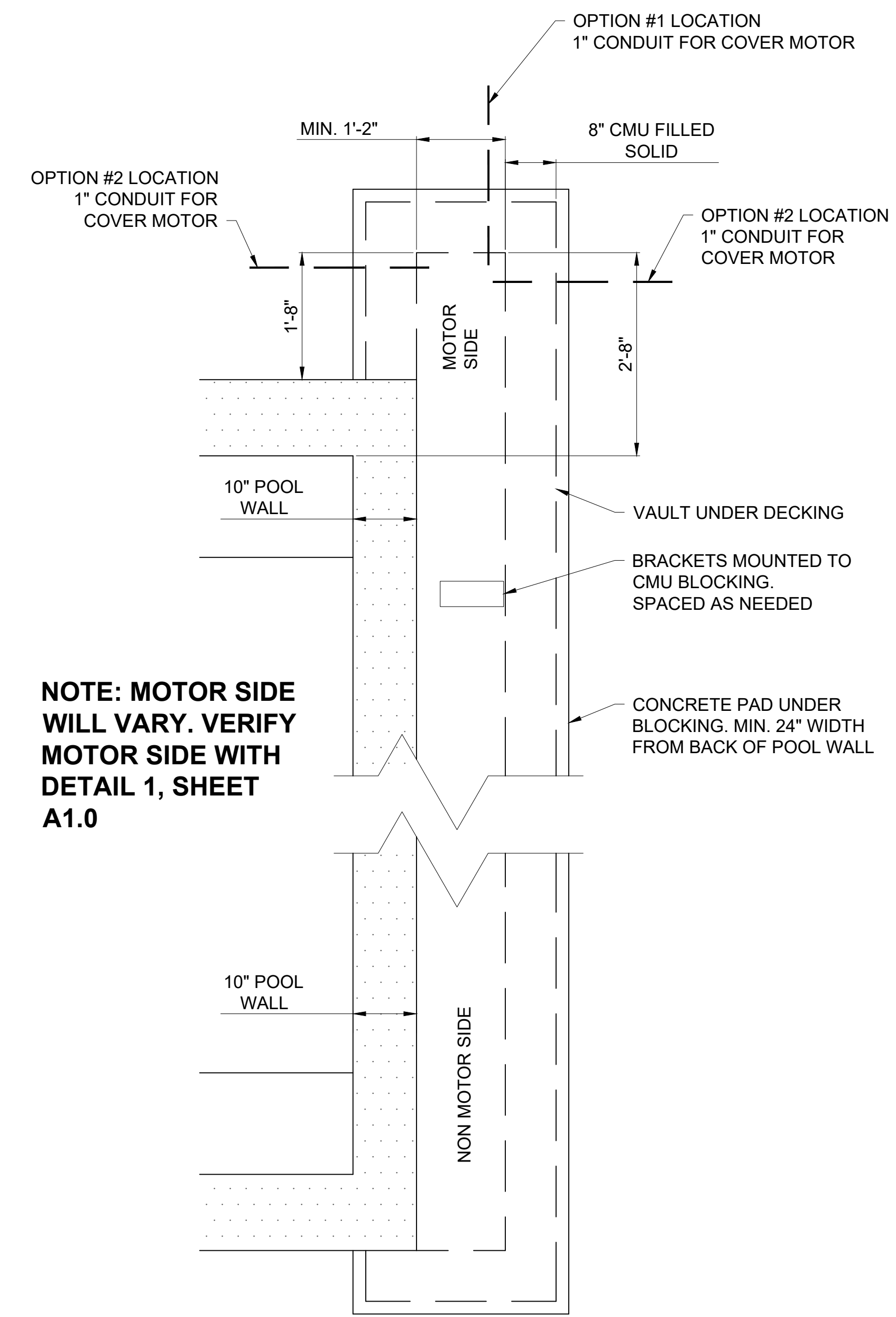
1 TYPICAL COVER VAULT DIMENSIONS SCALE: 3/4" = 1'-0"
