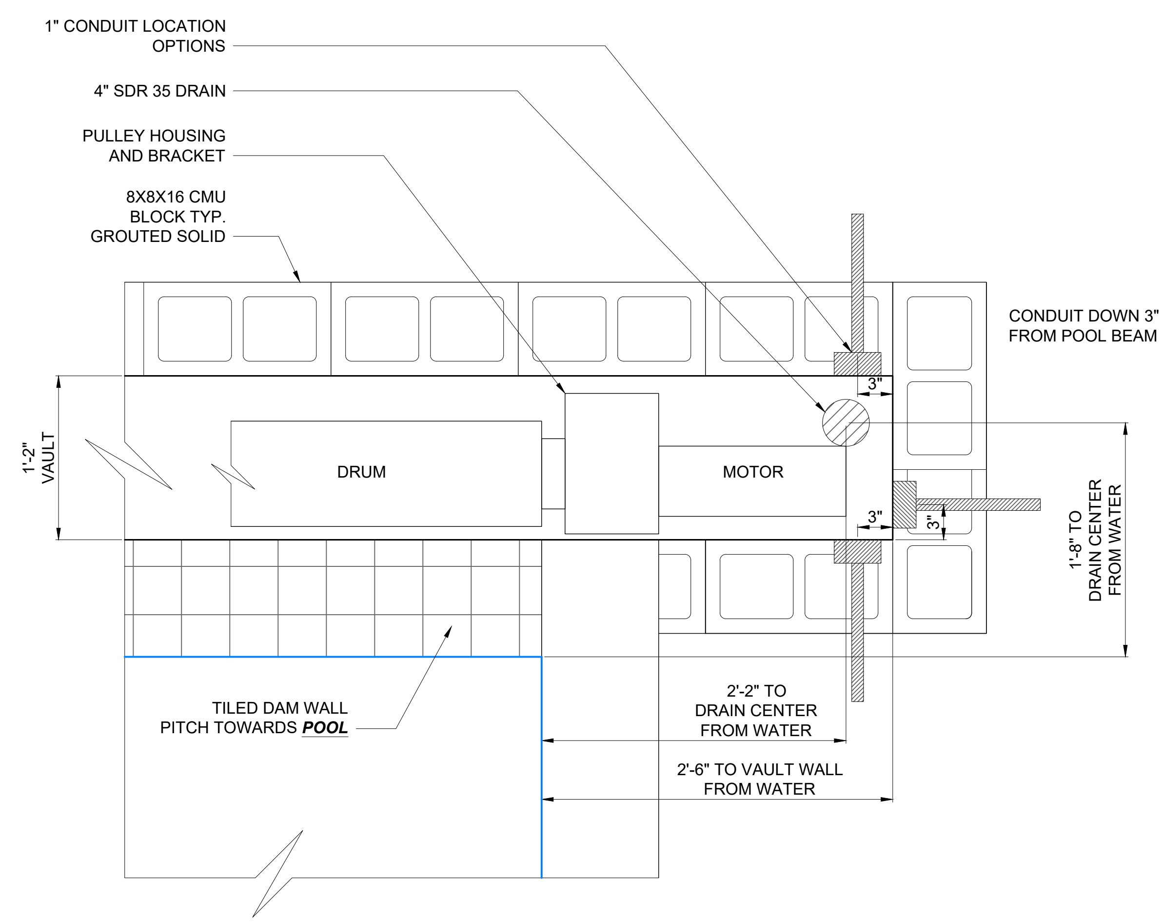
3 AUTO COVER VAULT DETAILS SCALE: 3/4" = 1'-0"
