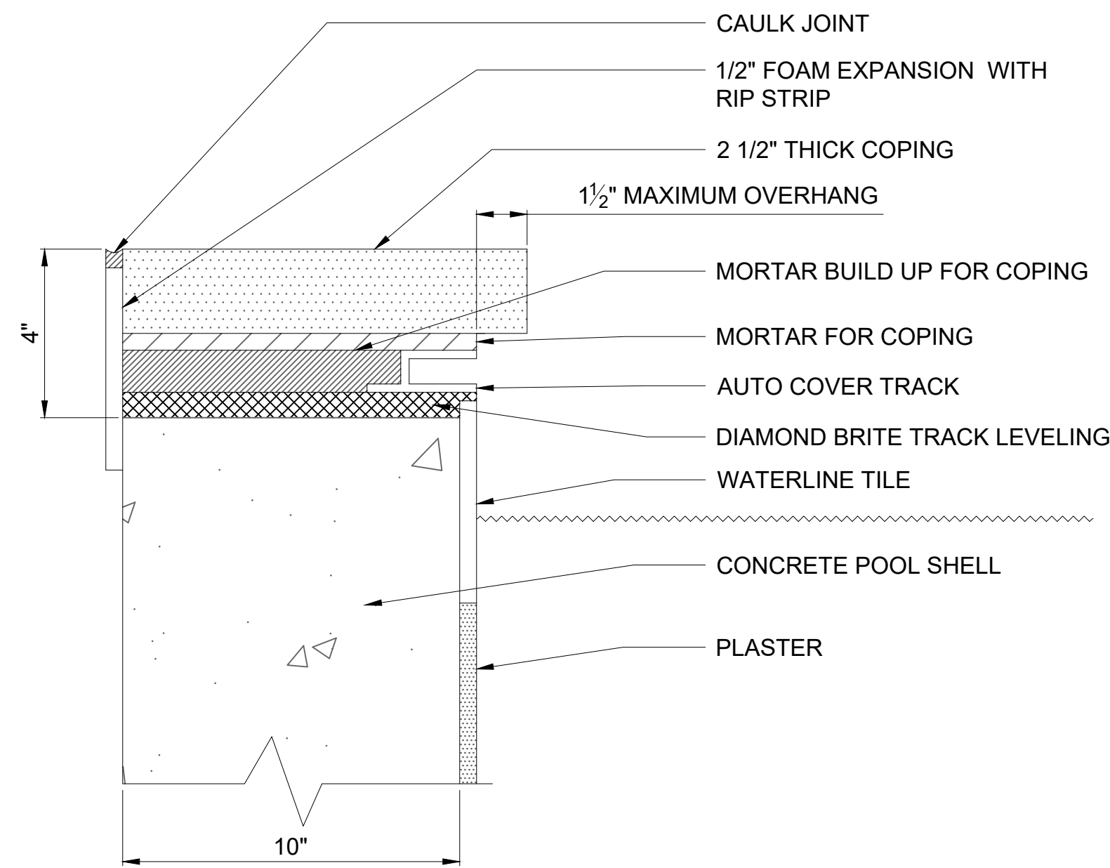
2 COPING SECTION WITH AUTO COVER TRACK SCALE: 3" = 1'-0"
