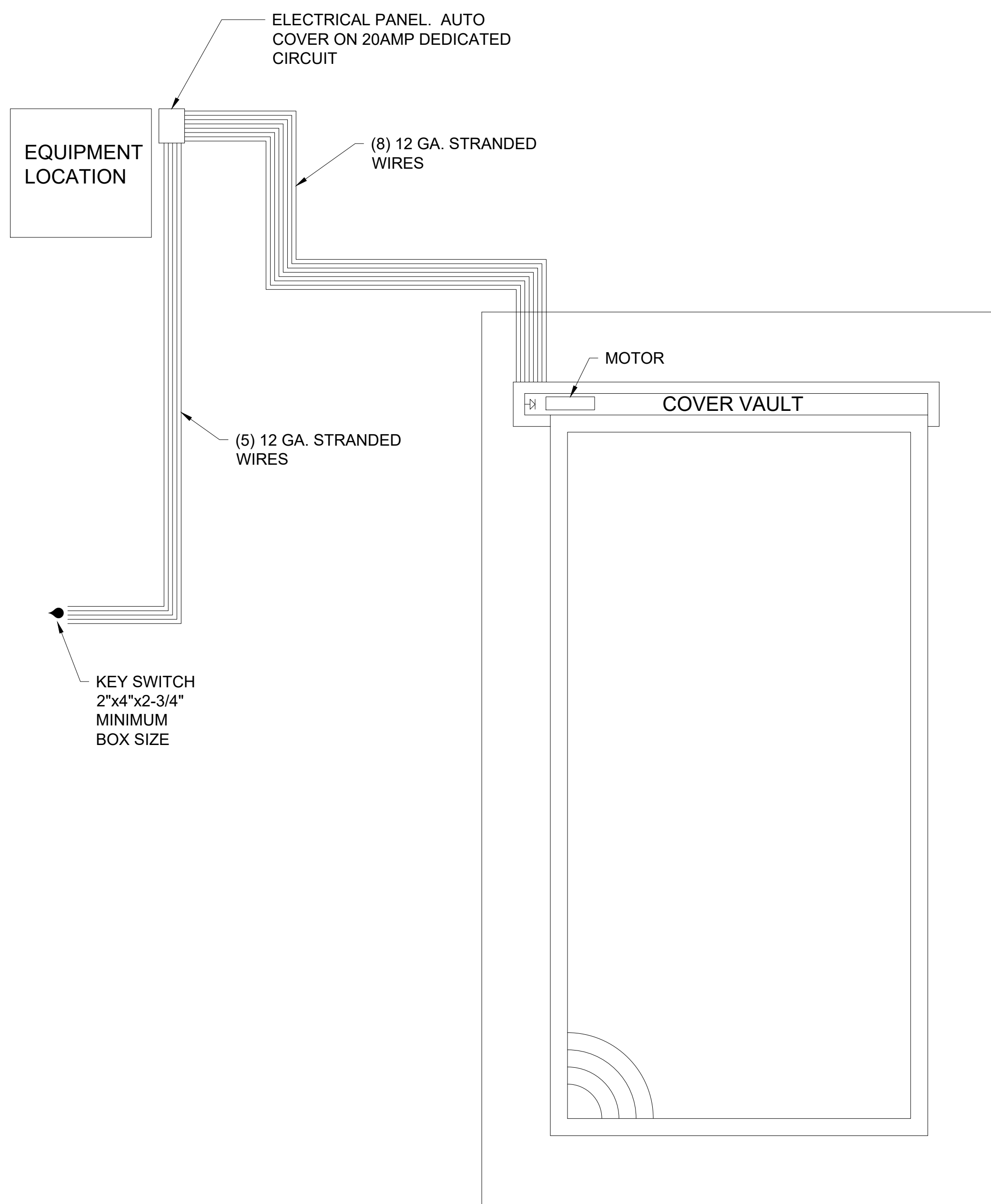
1 AUTO COVER WITHOUT SHUTOFF CONTROLLER SCALE: 3/8" = 1'-0"
