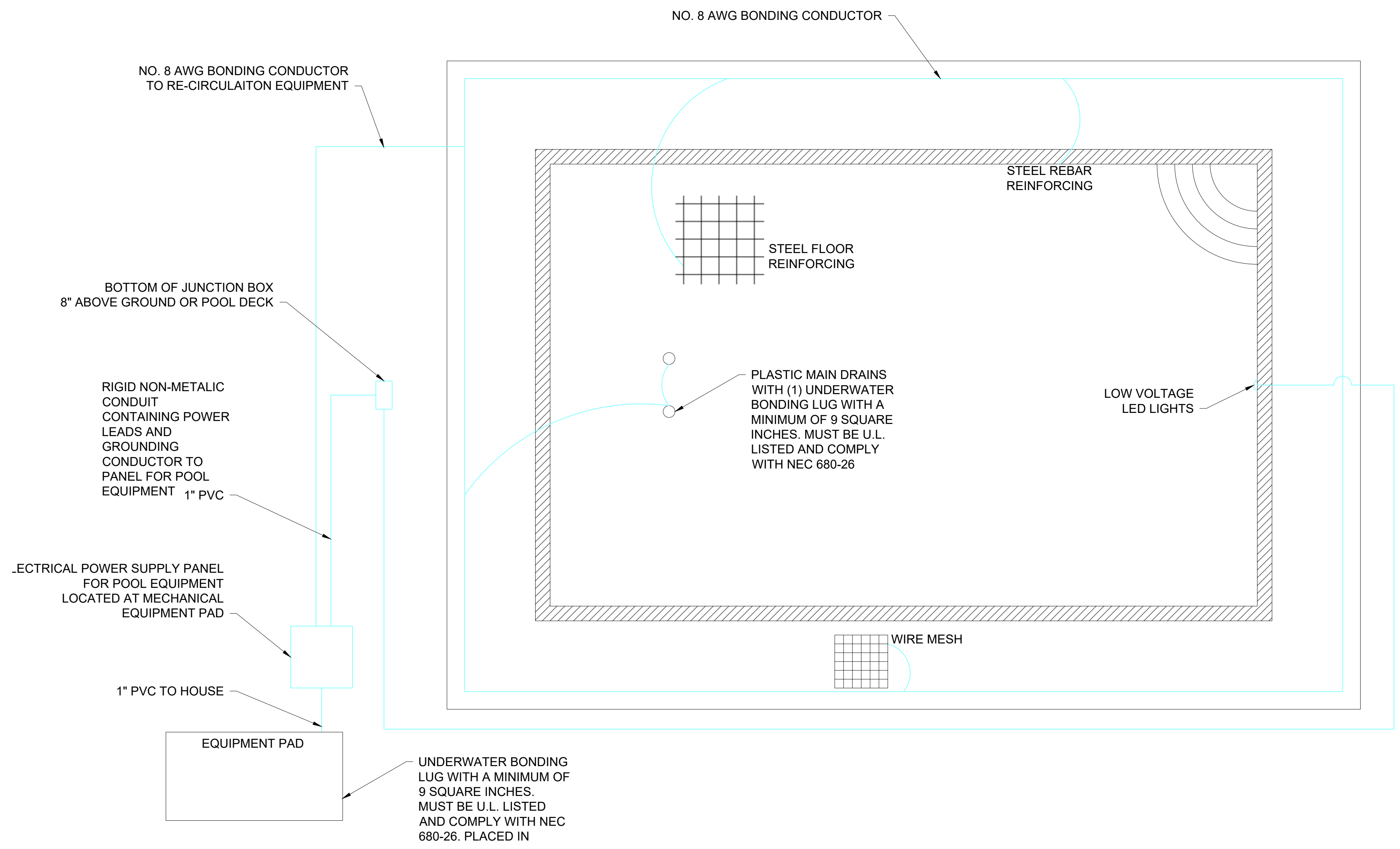
1 BONDING SCHEMATIC PLAN SCALE: 1/4" = 1'-0"
