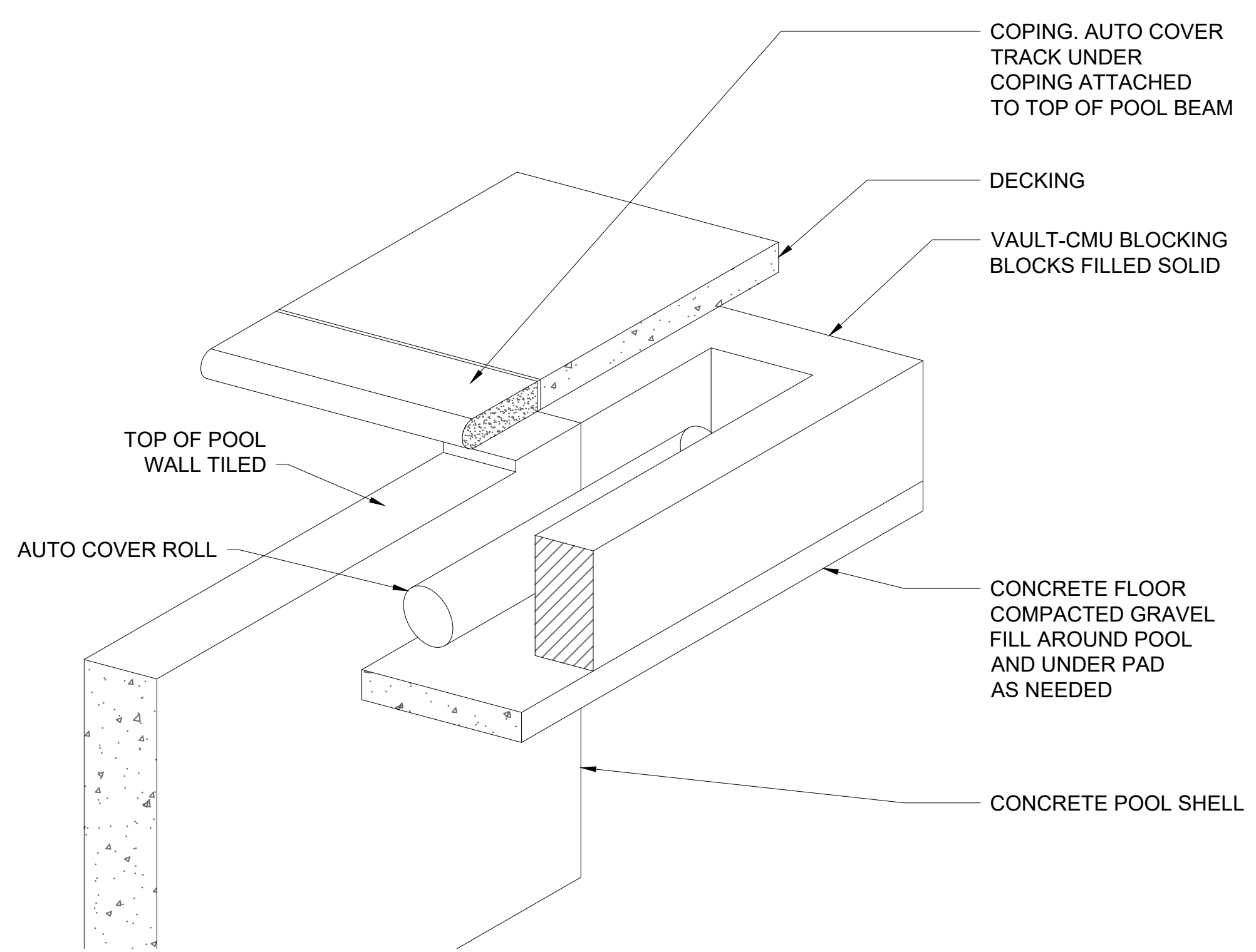
2 AUTO COVER VAULT ISOMETRIC SCALE: 3/4" = 1'-0"
